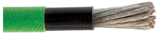
RG Flex L4, 4/0 AWG
